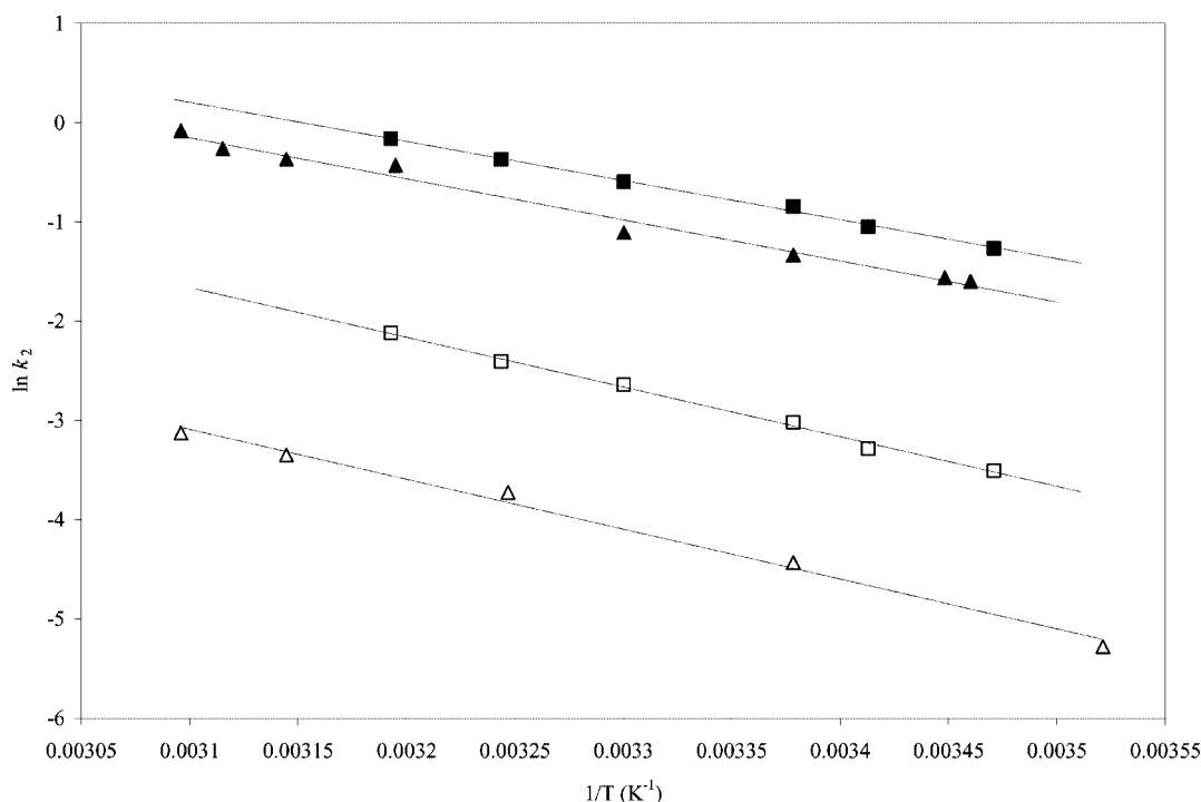
Figure 2. Arrhenius plots for the epoxidation of cis -4-methyl-2-pentene ( 2cis , ■)/ trans -4-methyl-2-pentene ( 2trans , □) and cis -2,2-dimethyl-3-hexene ( 6cis , ▲)/ trans -2,2-dimethyl-3-hexene ( 6trans , △) by 1 in dried acetone.
