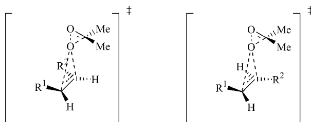
Figure 1. Representation of the spiro transition states for epoxidation of cis - and trans -alkenes by dimethyldioxirane ( 1 ).
